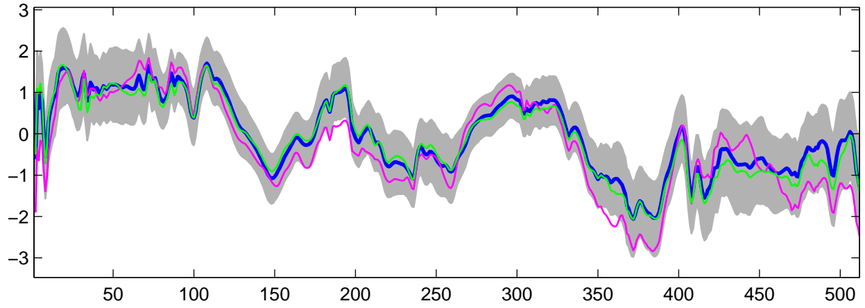
Estimated U_{14}(t) using G-WFMM: Normal data, run 1
