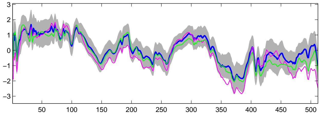
Estimated U_{14}(t) using R-WFMM: Normal data, run 1
