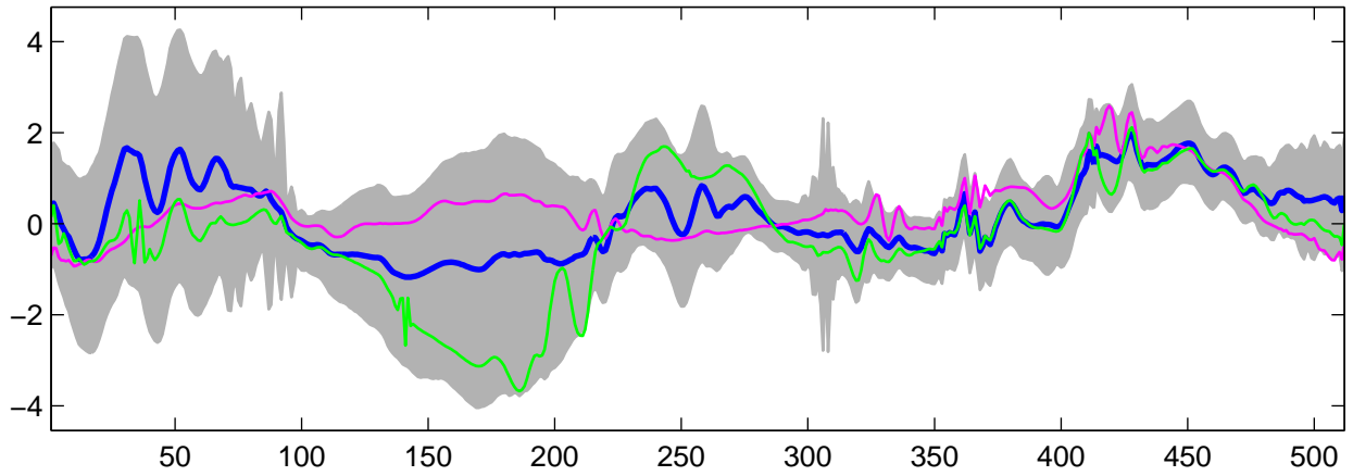
Estimated U_{14}(t) using G-WFMM: t_1 data, run 1
