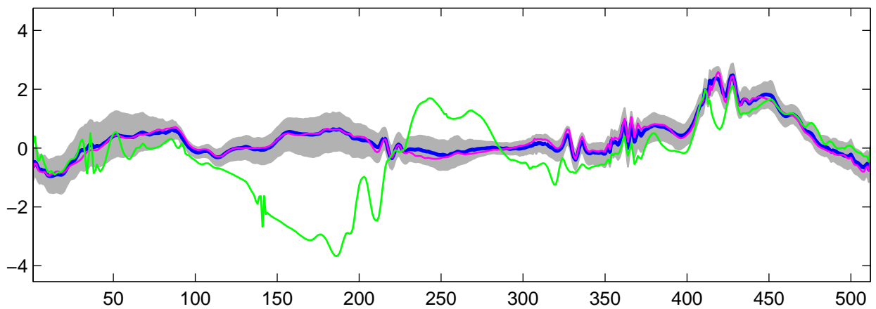
Estimated U_{14}(t) using R-WFMM: t_1 data, run 1
