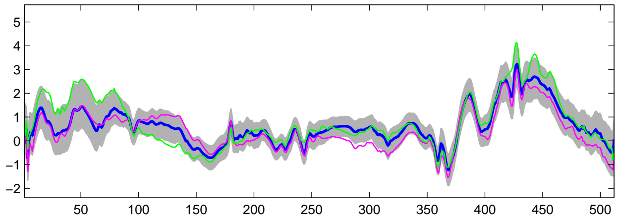
Estimated U_{14}(t) using R-WFMM: t_2 data, run 1
