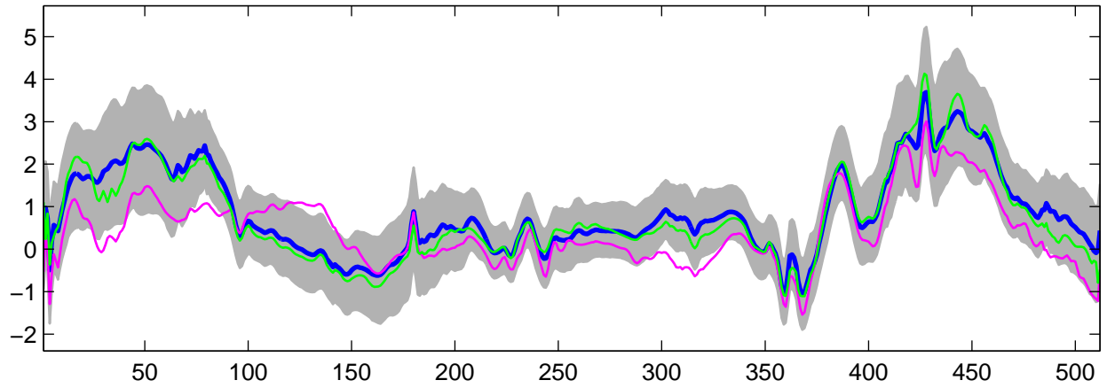
Estimated U_{14}(t) using G-WFMM: t_2 data, run 1
