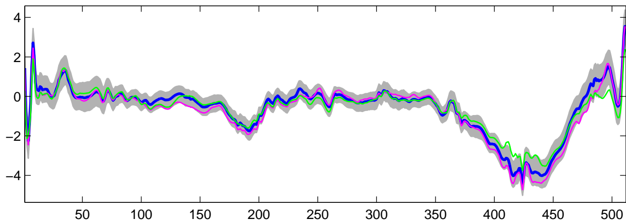
Estimated U_{14}(t) using R-WFMM: t_3 data, run 1
