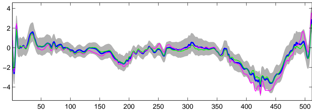
Estimated U_{14}(t) using G-WFMM: t_3 data, run 1
