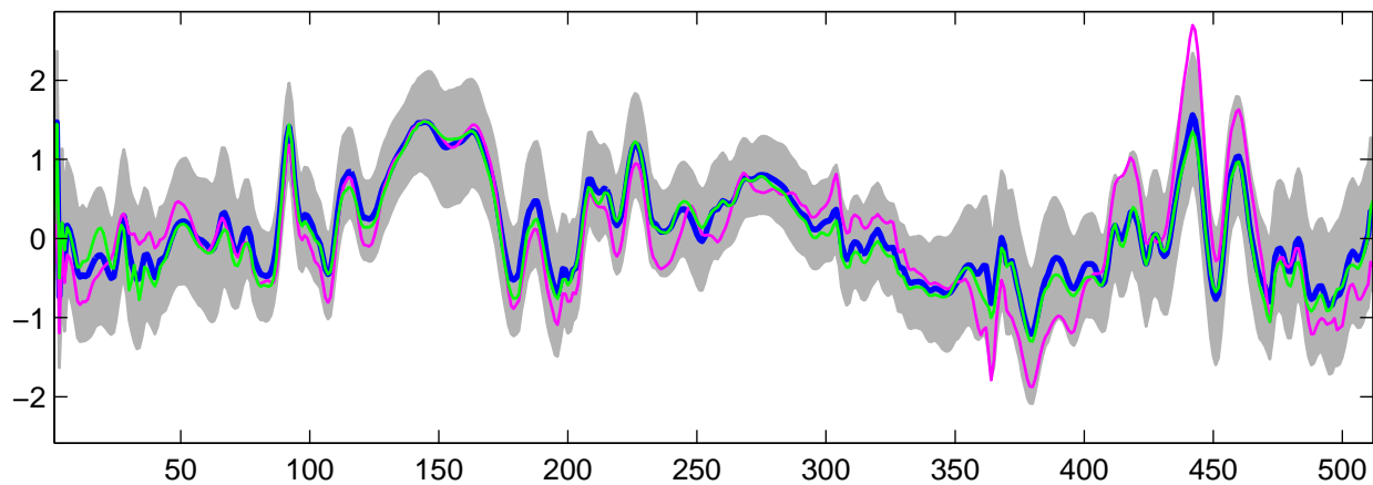
Estimated U_{15}(t) using G-WFMM: DE data, run 1
