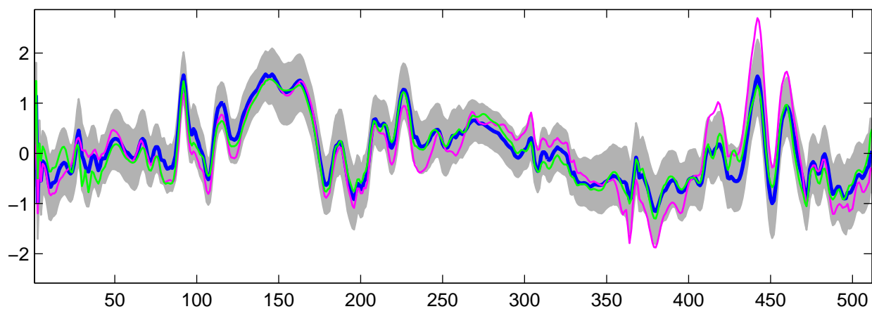
Estimated U_{15}(t) using R-WFMM: DE data, run 1
