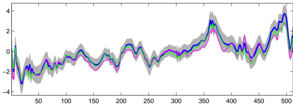
Estimated U_{15}(t) using R-WFMM: Normal data, run 1
