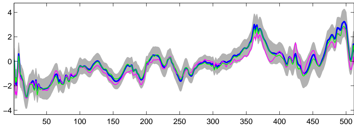
Estimated U_{15}(t) using G-WFMM: Normal data, run 1
