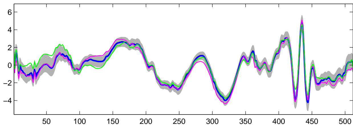
Estimated U_{15}(t) using R-WFMM: t_2 data, run 1
