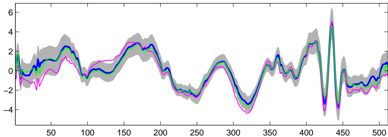
Estimated U_{15}(t) using G-WFMM: t_2 data, run 1
