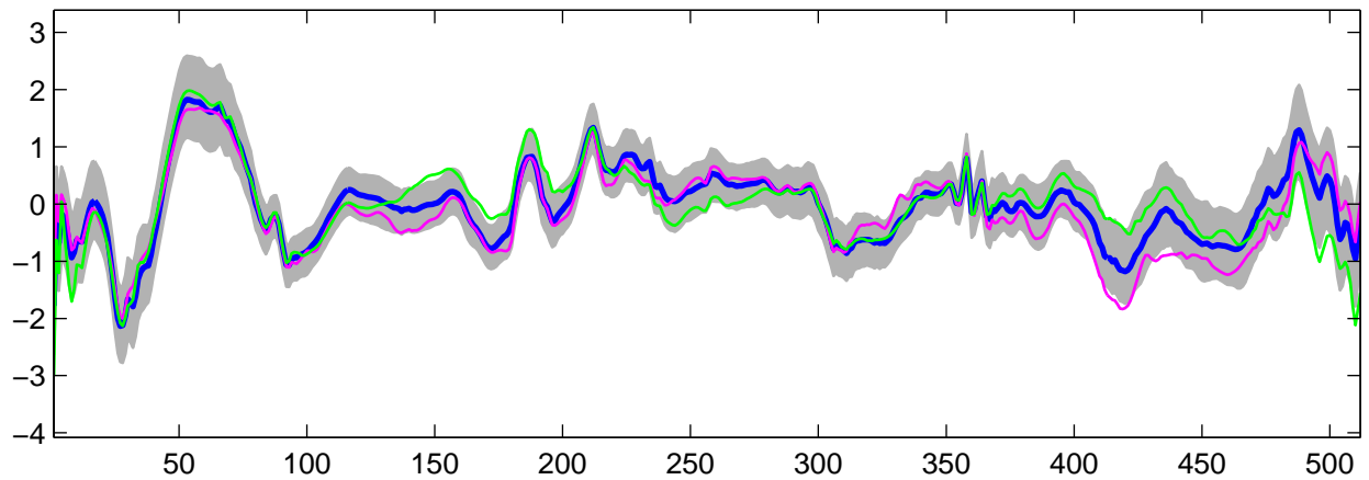
Estimated U_{15}(t) using R-WFMM: t_3 data, run 1
