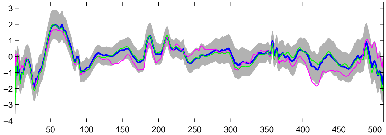
Estimated U_{15}(t) using G-WFMM: t_3 data, run 1
