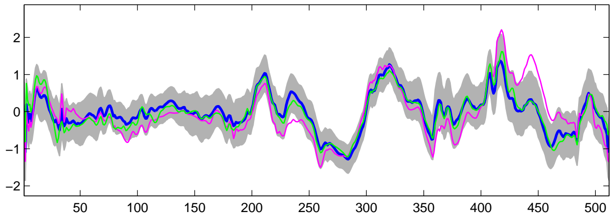
Estimated U_{16}(t) using R-WFMM: DE data, run 1
