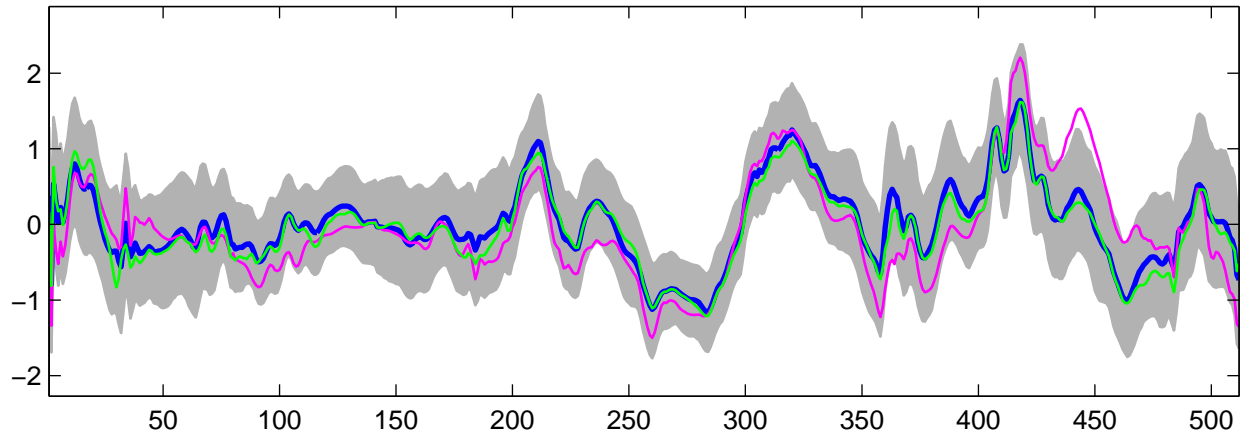
Estimated U_{16}(t) using G-WFMM: DE data, run 1
