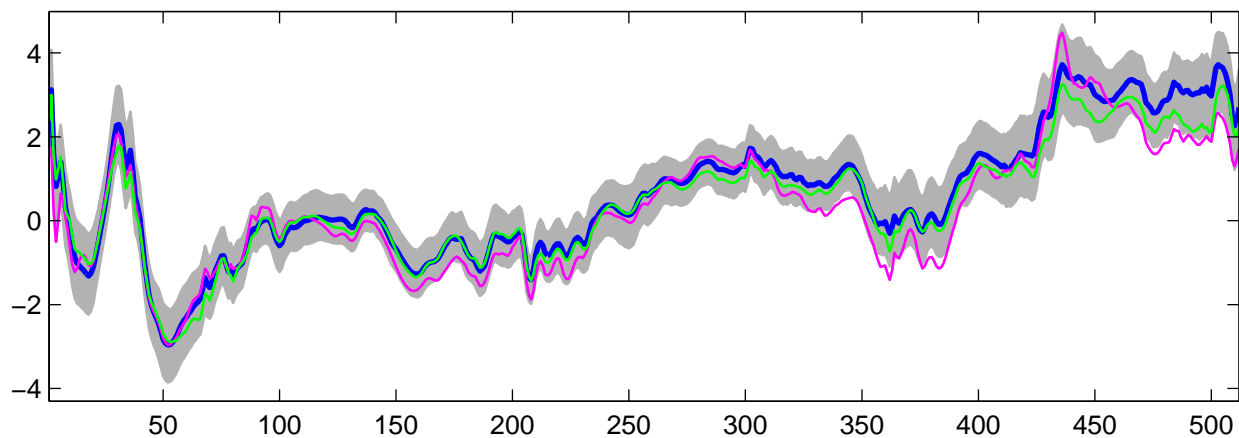
Estimated U_{16}(t) using R-WFMM: Normal data, run 1
