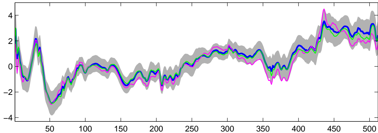
Estimated U_{16}(t) using G-WFMM: Normal data, run 1
