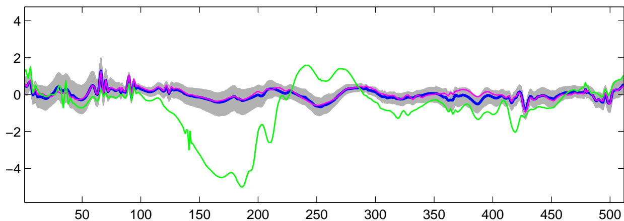
Estimated U_{16}(t) using R-WFMM: t_1 data, run 1
