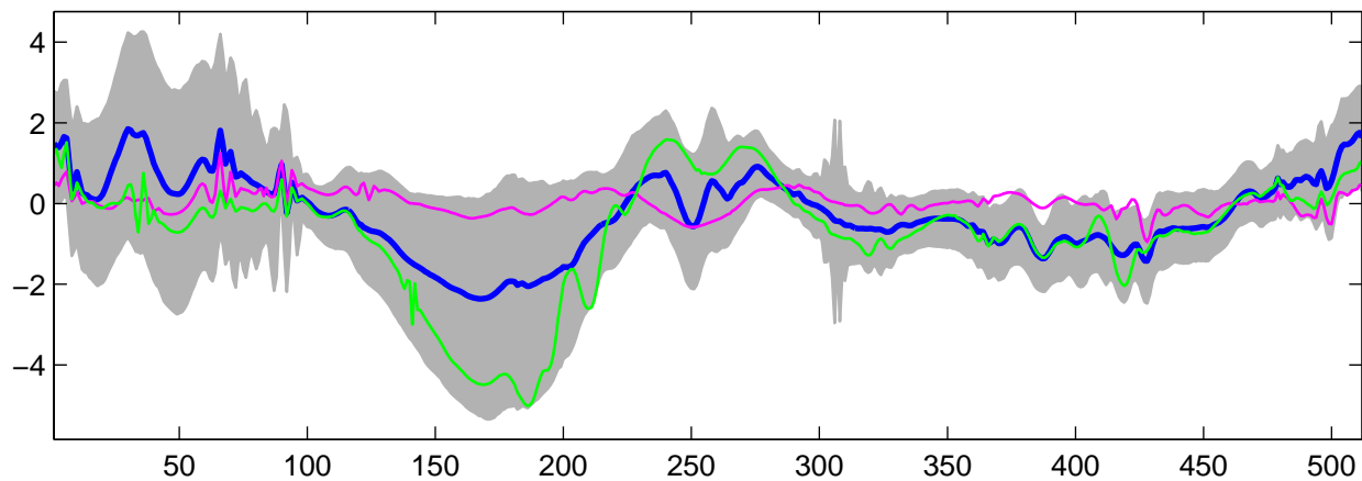
Estimated U_{16}(t) using G-WFMM: t_1 data, run 1
