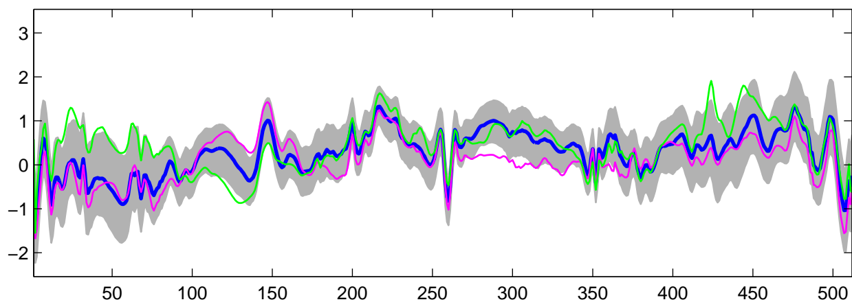
Estimated U_{16}(t) using R-WFMM: t_2 data, run 1
