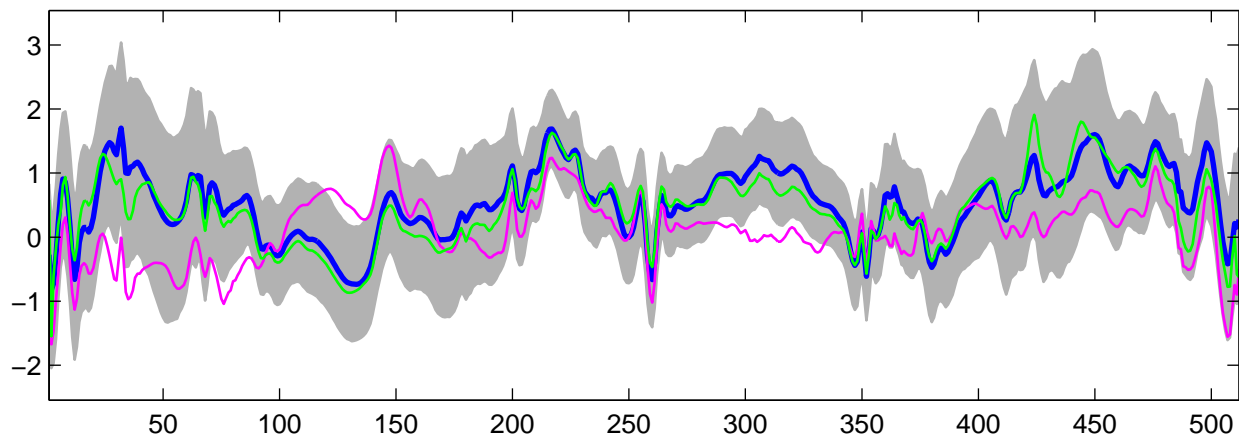
Estimated U_{16}(t) using G-WFMM: t_2 data, run 1
