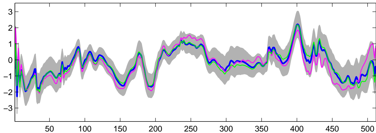
Estimated U_{16}(t) using G-WFMM: t_3 data, run 1
