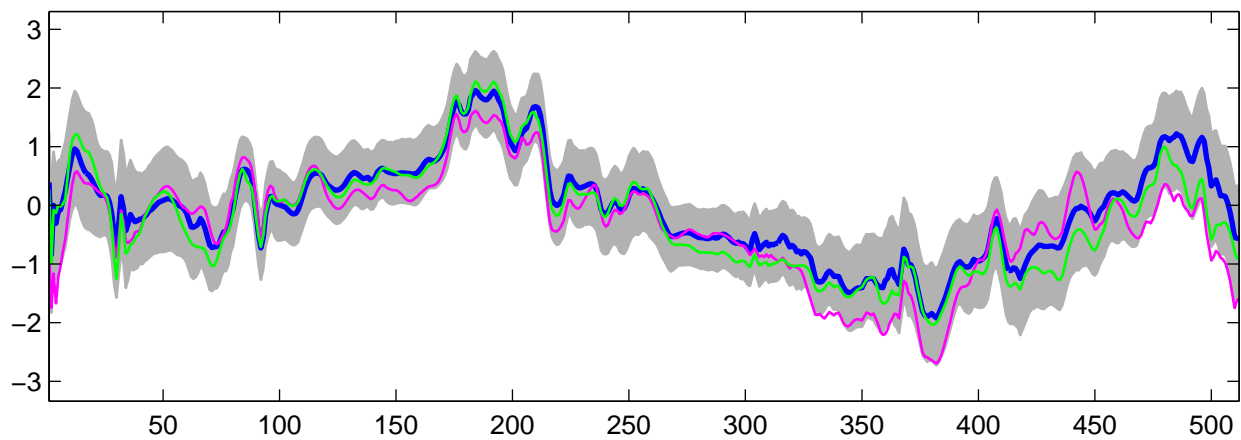
Estimated U_{17}(t) using R-WFMM: Normal data, run 1
