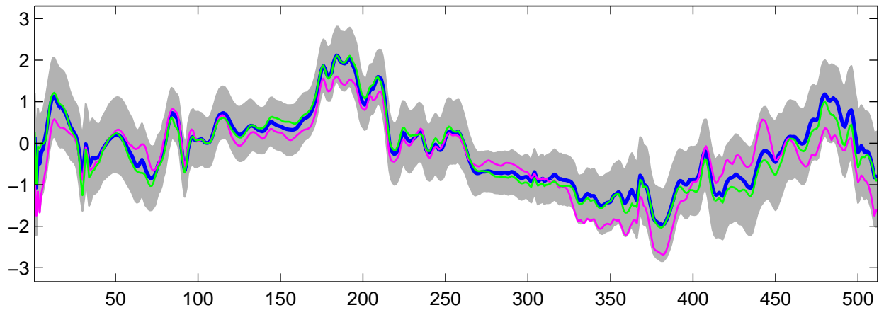
Estimated U_{17}(t) using G-WFMM: Normal data, run 1
