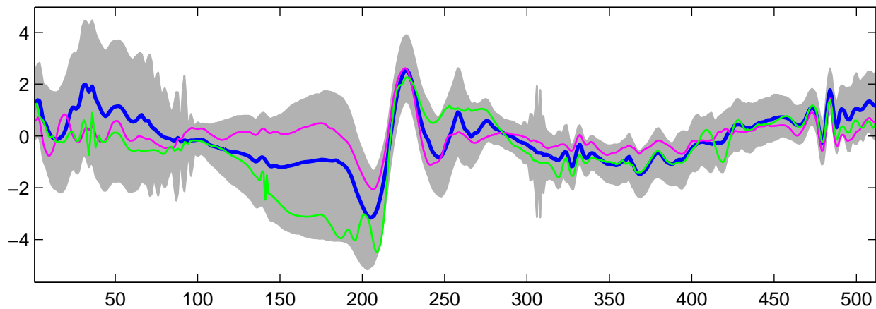
Estimated U_{17}(t) using G-WFMM: t_1 data, run 1
