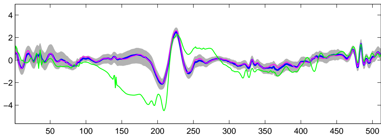
Estimated U_{17}(t) using R-WFMM: t_1 data, run 1
