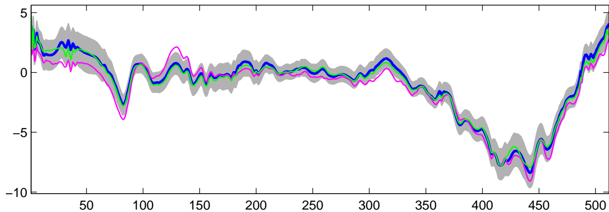
Estimated U_{17}(t) using G-WFMM: t_2 data, run 1
