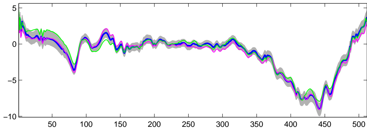
Estimated U_{17}(t) using R-WFMM: t_2 data, run 1
