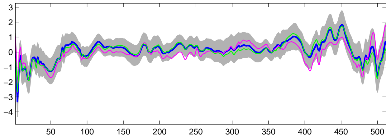
Estimated U_{17}(t) using G-WFMM: t_3 data, run 1
