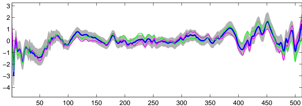
Estimated U_{17}(t) using R-WFMM: t_3 data, run 1
