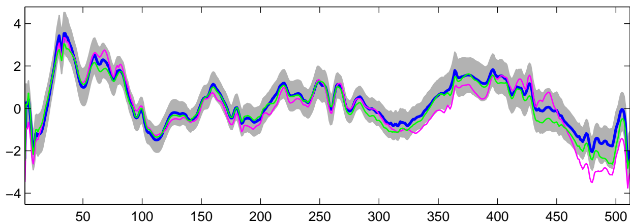
Estimated U_{18}(t) using R-WFMM: Normal data, run 1
