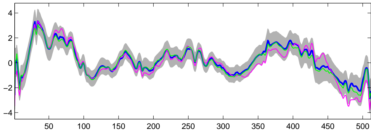
Estimated U_{18}(t) using G-WFMM: Normal data, run 1
