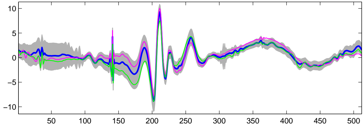
Estimated U_{18}(t) using G-WFMM: t_1 data, run 1
