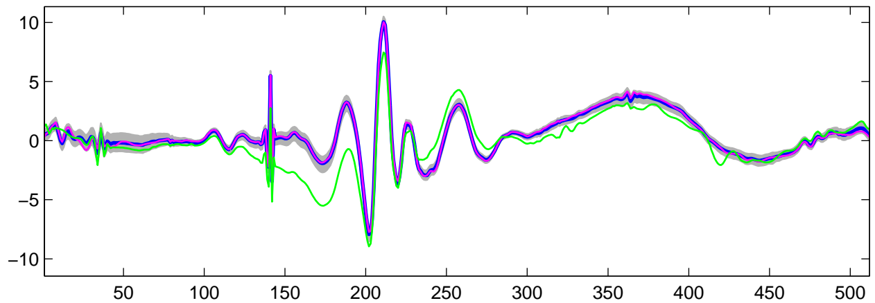
Estimated U_{18}(t) using R-WFMM: t_1 data, run 1
