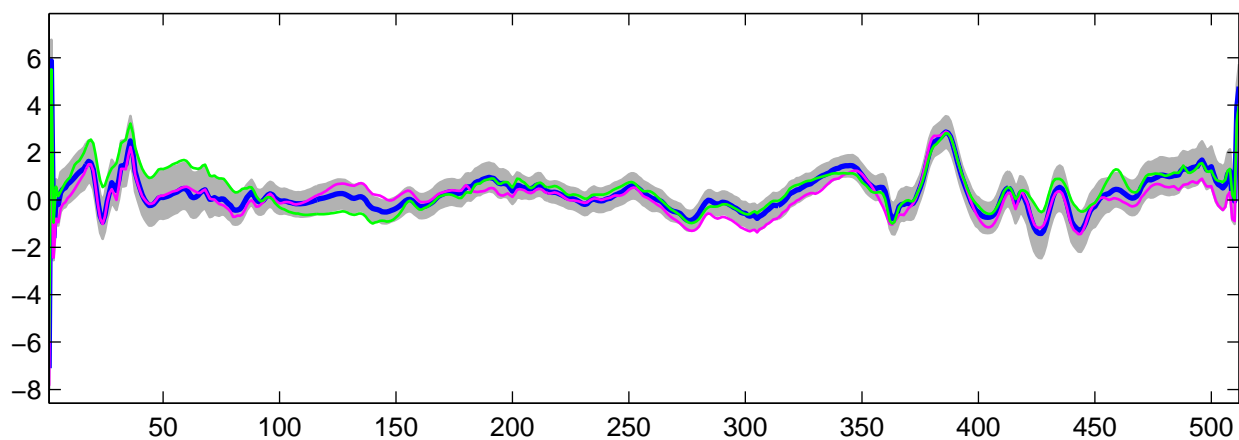
Estimated U_{18}(t) using R-WFMM: t_2 data, run 1
