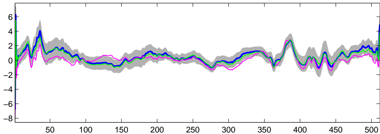
Estimated U_{18}(t) using G-WFMM: t_2 data, run 1
