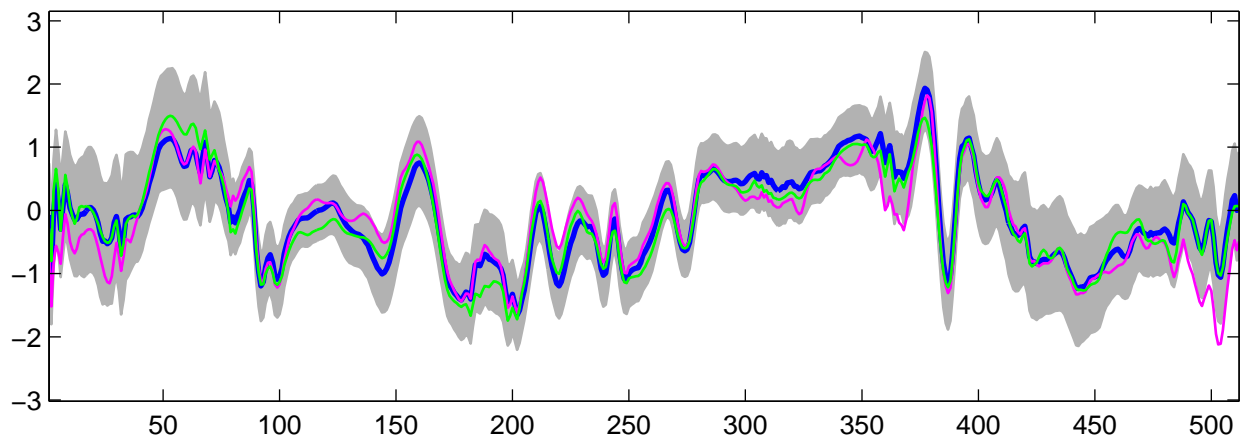
Estimated U_{19}(t) using R-WFMM: DE data, run 1
