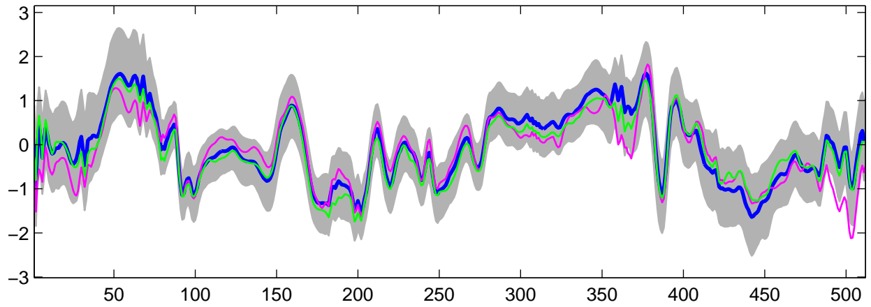
Estimated U_{19}(t) using G-WFMM: DE data, run 1
