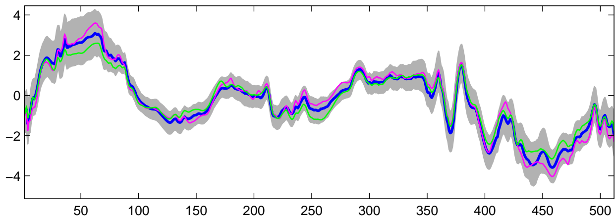
Estimated U_{19}(t) using R-WFMM: Normal data, run 1
