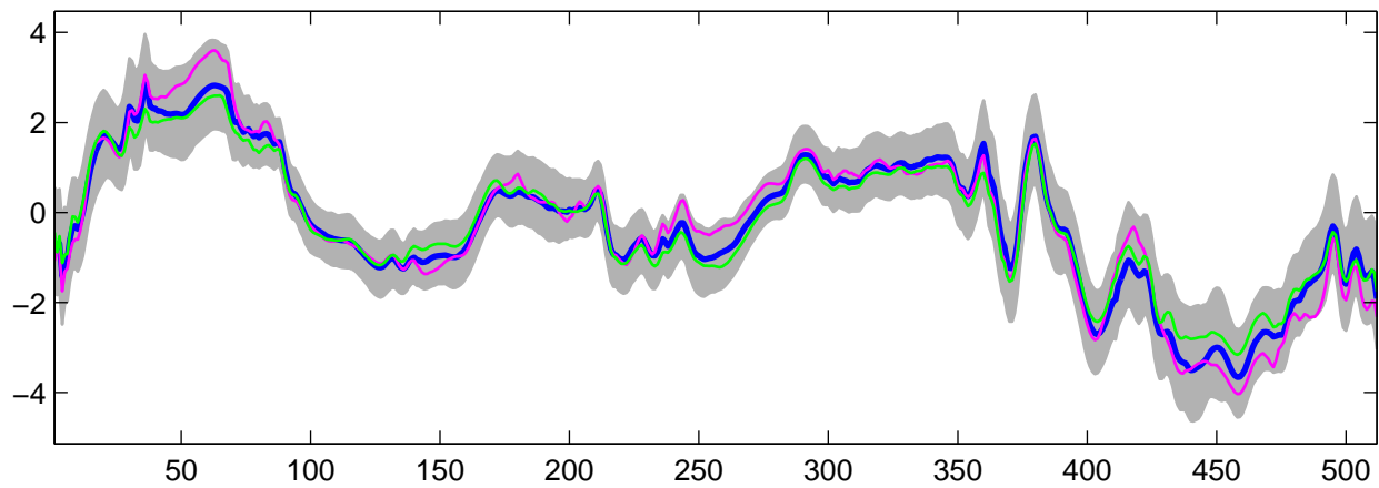
Estimated U_{19}(t) using G-WFMM: Normal data, run 1
