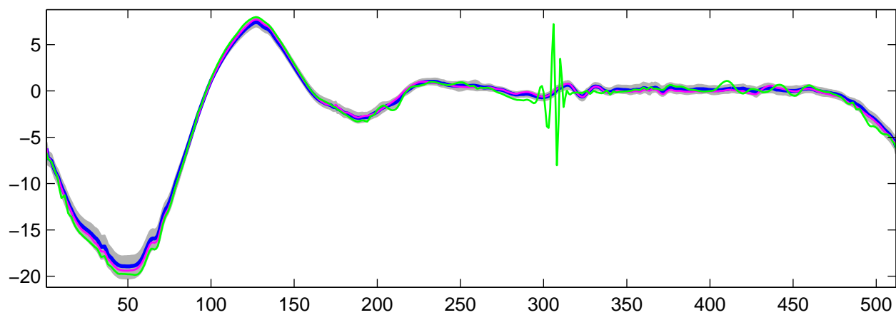
Estimated U_{19}(t) using R-WFMM: t_1 data, run 1
