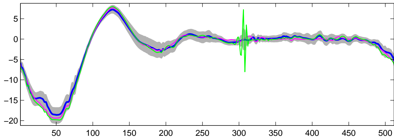
Estimated U_{19}(t) using G-WFMM: t_1 data, run 1
