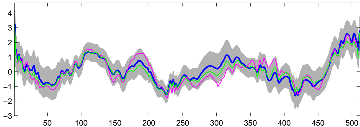
Estimated U_{19}(t) using G-WFMM: t_3 data, run 1
