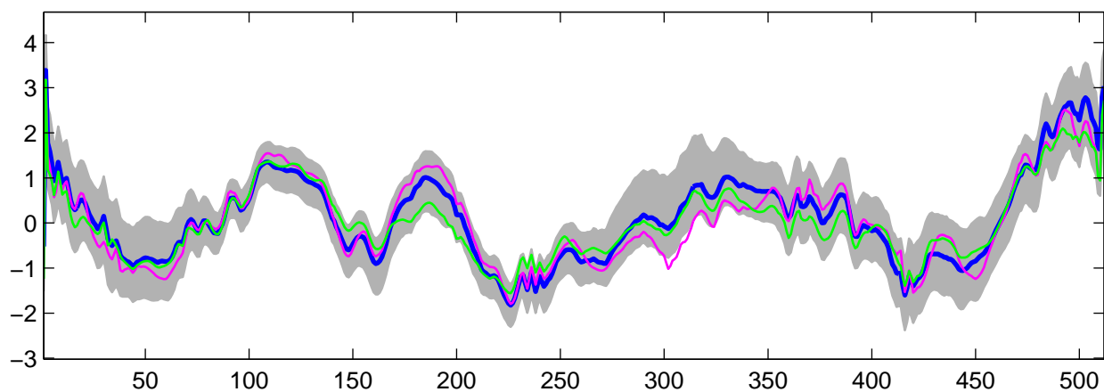
Estimated U_{19}(t) using R-WFMM: t_3 data, run 1
