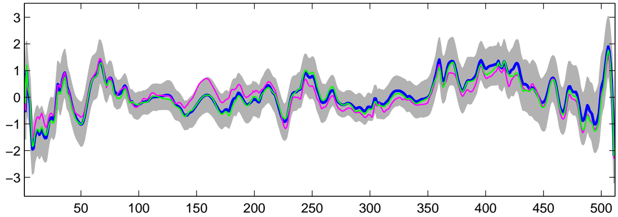
Estimated U_1(t) using G-WFMM: Normal data, run 1
