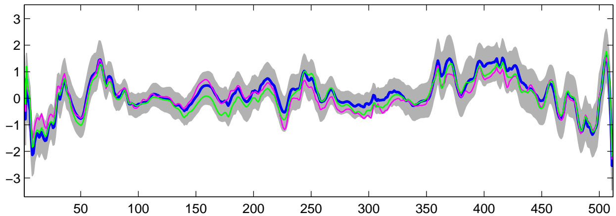
Estimated U_1(t) using R-WFMM: Normal data, run 1
