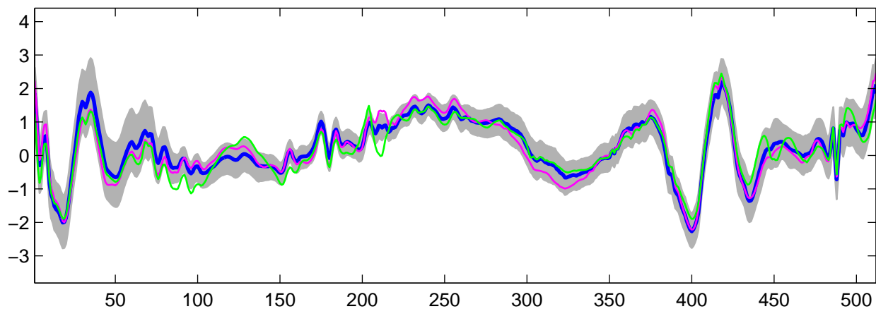
Estimated U_1(t) using R-WFMM: t_2 data, run 1
