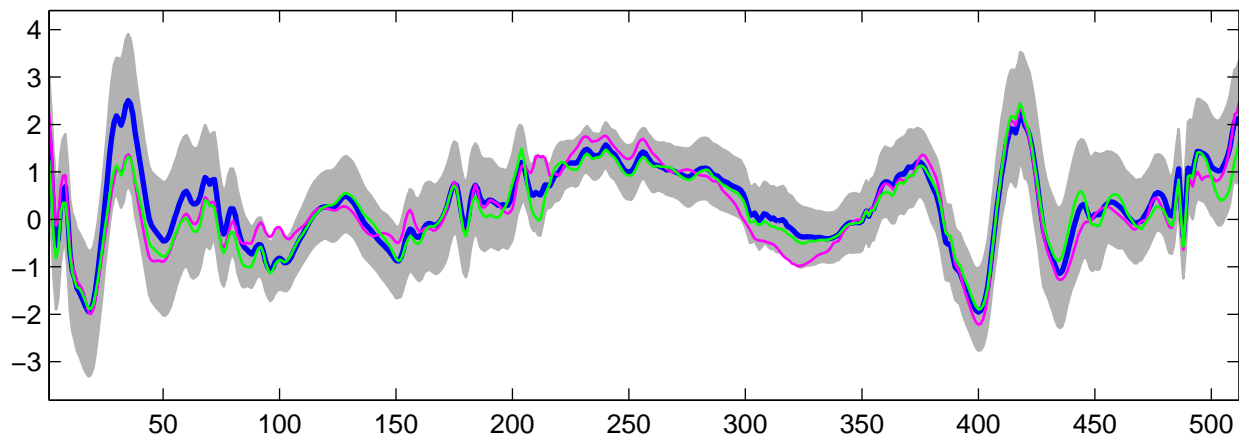
Estimated U_1(t) using G-WFMM: t_2 data, run 1
