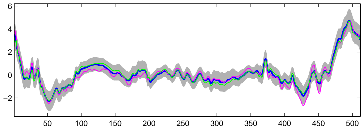
Estimated U_1(t) using G-WFMM: t_3 data, run 1
