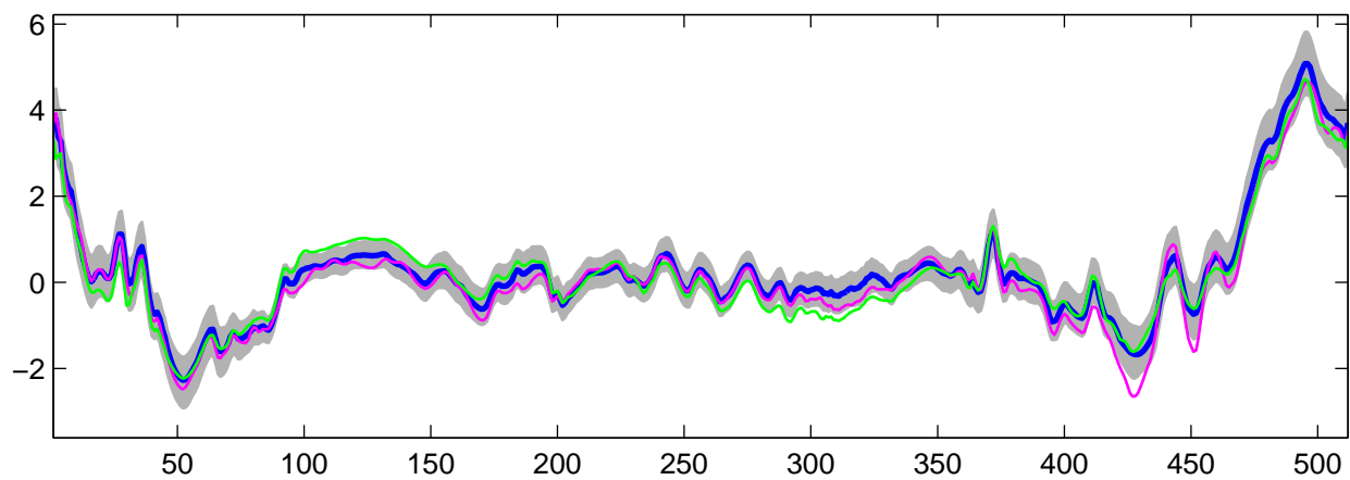
Estimated U_1(t) using R-WFMM: t_3 data, run 1
