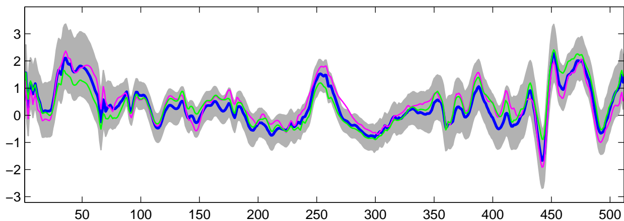
Estimated U_{20}(t) using R-WFMM: Normal data, run 1
