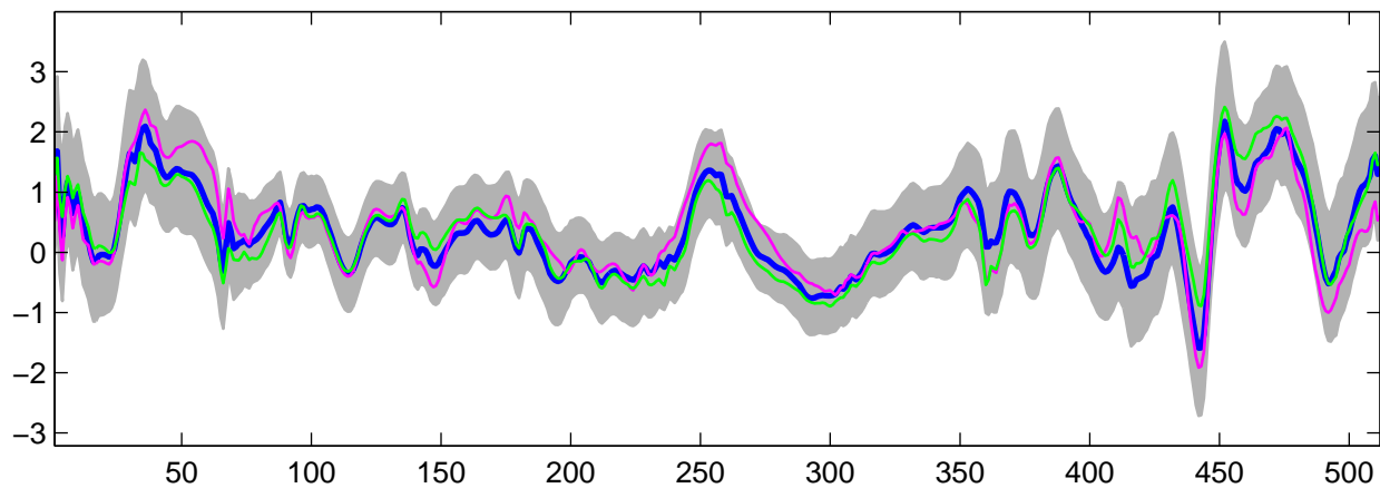
Estimated U_{20}(t) using G-WFMM: Normal data, run 1
