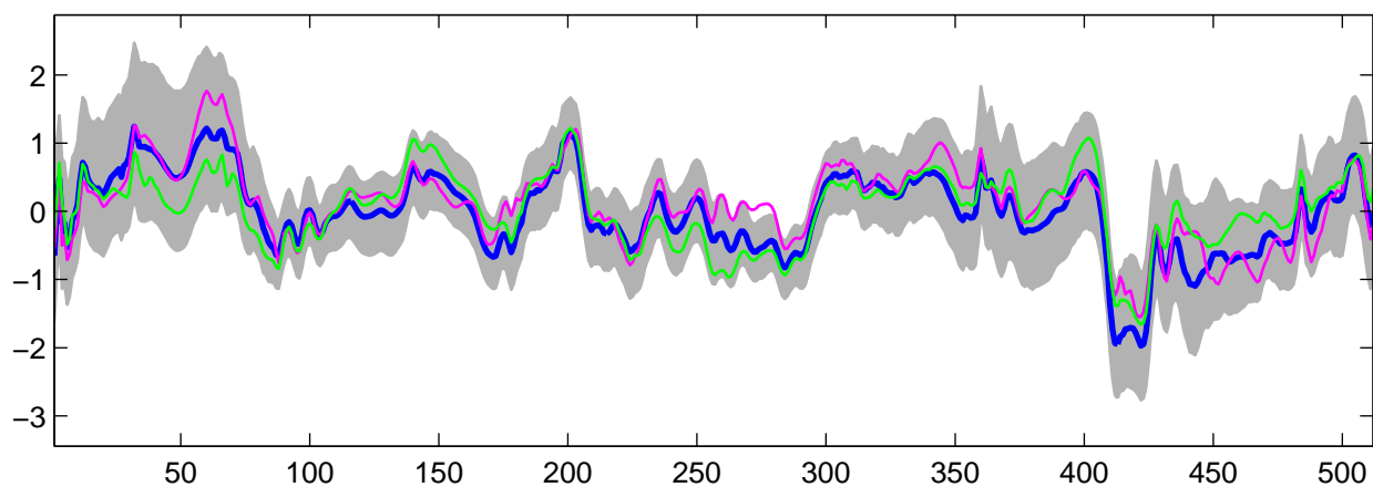
Estimated U_{21}(t) using R-WFMM: Normal data, run 1
