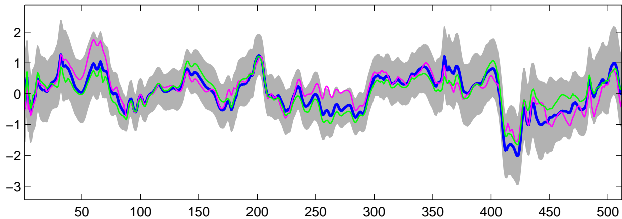
Estimated U_{21}(t) using G-WFMM: Normal data, run 1
