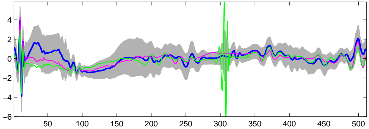
Estimated U_{21}(t) using G-WFMM: t_1 data, run 1
