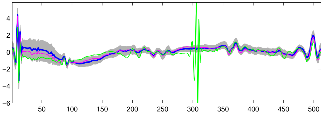
Estimated U_{21}(t) using R-WFMM: t_1 data, run 1
