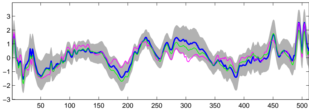
Estimated U_{21}(t) using G-WFMM: t_3 data, run 1
