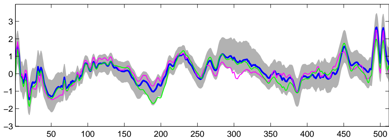
Estimated U_{21}(t) using R-WFMM: t_3 data, run 1
