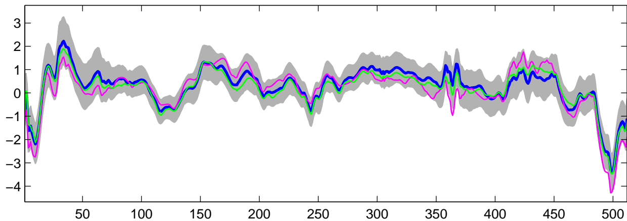
Estimated U_{22}(t) using G-WFMM: DE data, run 1
