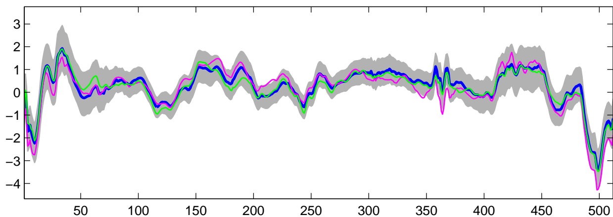
Estimated U_{22}(t) using R-WFMM: DE data, run 1
