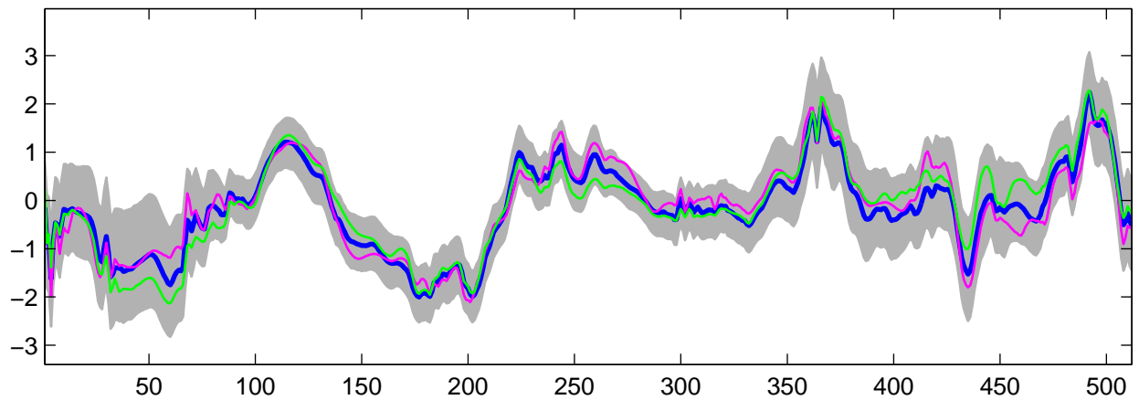
Estimated U_{22}(t) using R-WFMM: Normal data, run 1
