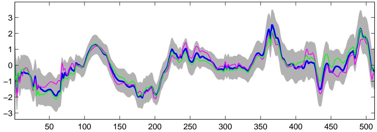
Estimated U_{22}(t) using G-WFMM: Normal data, run 1
