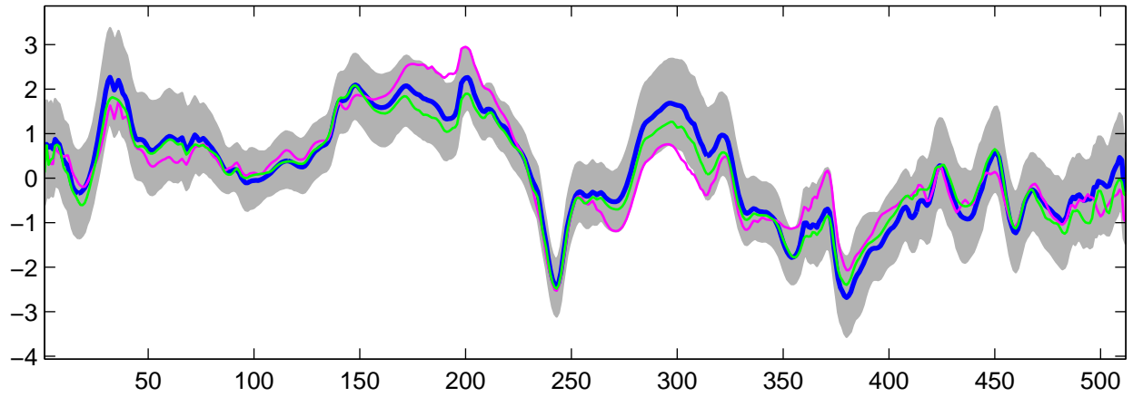
Estimated U_{22}(t) using G-WFMM: t_3 data, run 1
