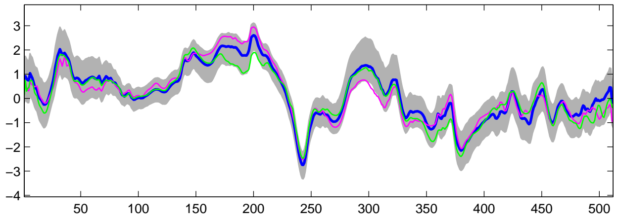
Estimated U_{22}(t) using R-WFMM: t_3 data, run 1
