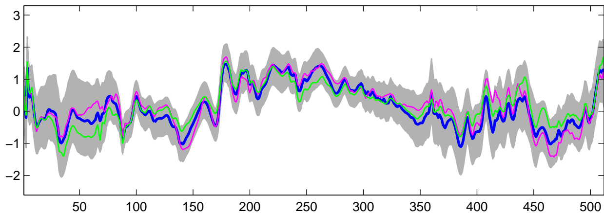
Estimated U_{23}(t) using R-WFMM: Normal data, run 1
