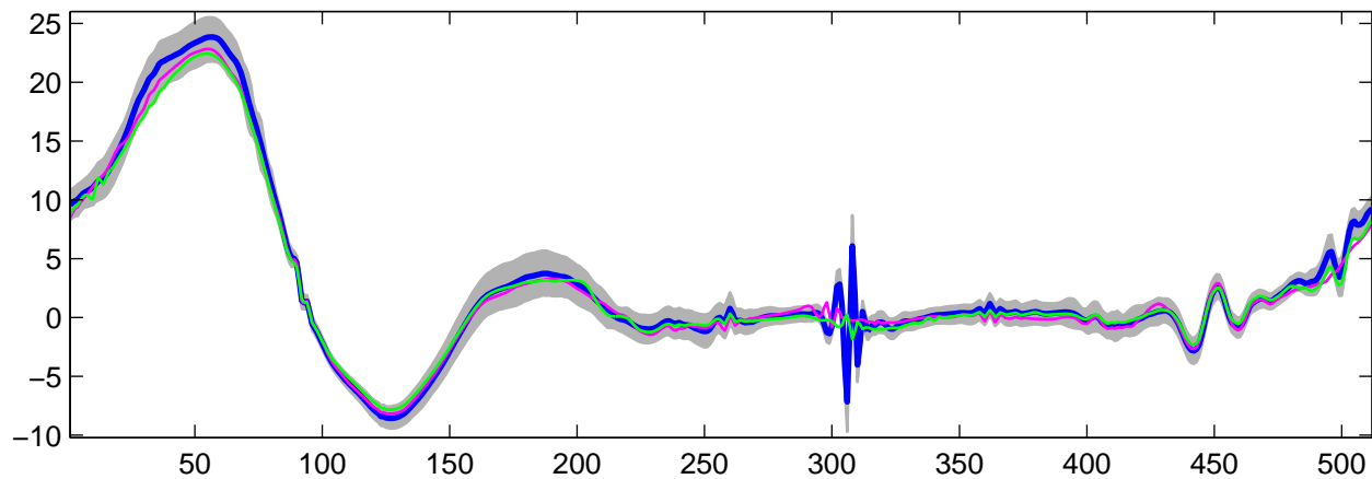
Estimated U_{23}(t) using G-WFMM: t_1 data, run 1
