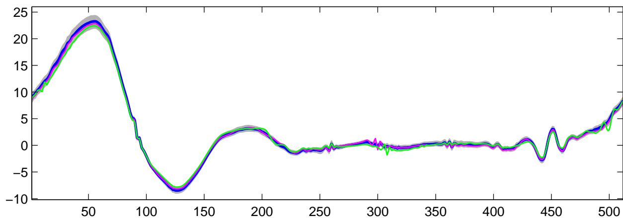
Estimated U_{23}(t) using R-WFMM: t_1 data, run 1
