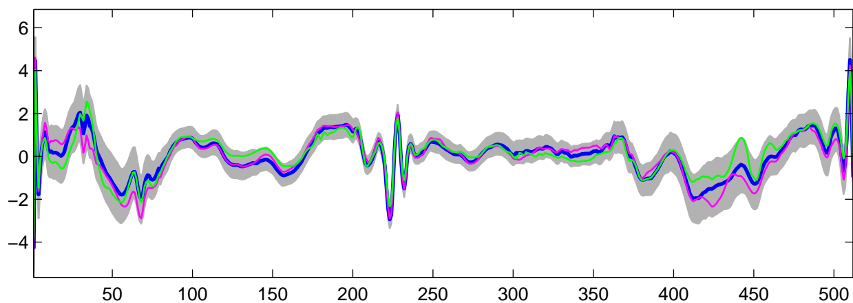
Estimated U_{23}(t) using R-WFMM: t_2 data, run 1
