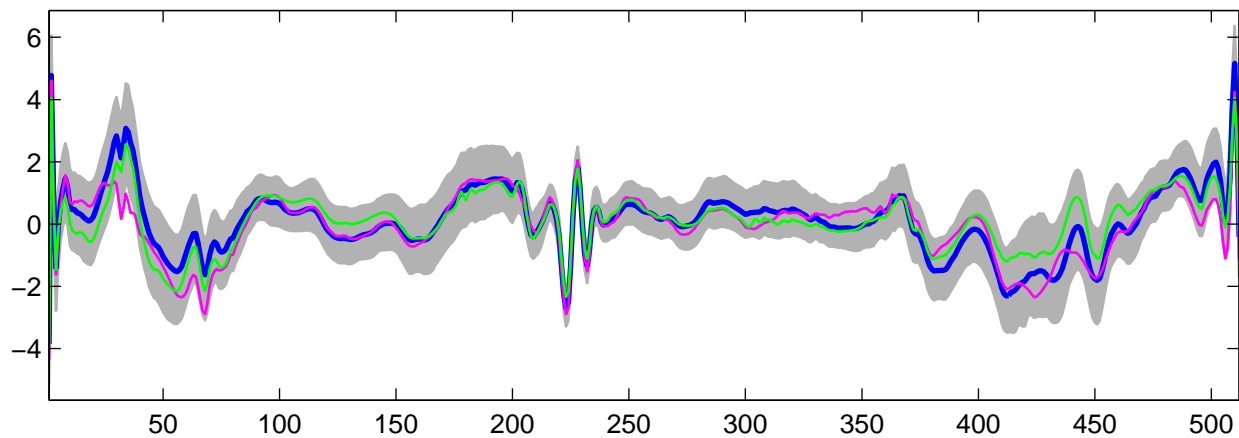
Estimated U_{23}(t) using G-WFMM: t_2 data, run 1
