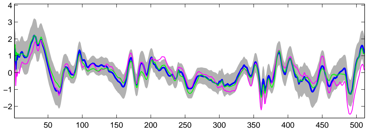
Estimated U_{24}(t) using R-WFMM: DE data, run 1
