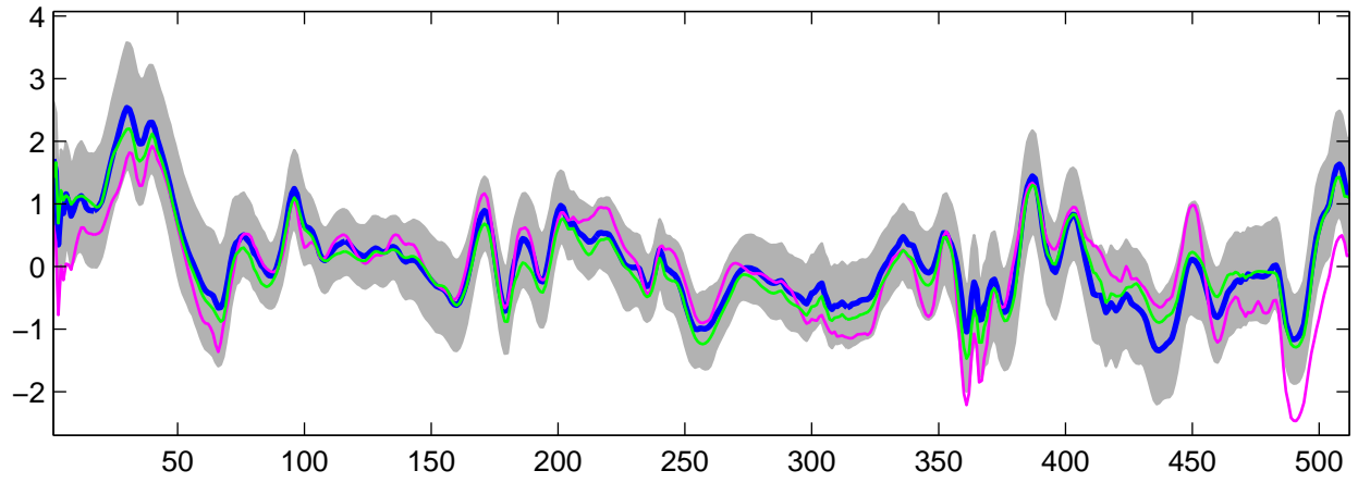
Estimated U_{24}(t) using G-WFMM: DE data, run 1
