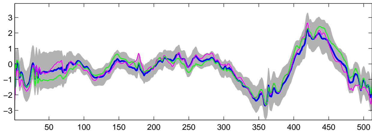
Estimated U_{24}(t) using R-WFMM: Normal data, run 1
