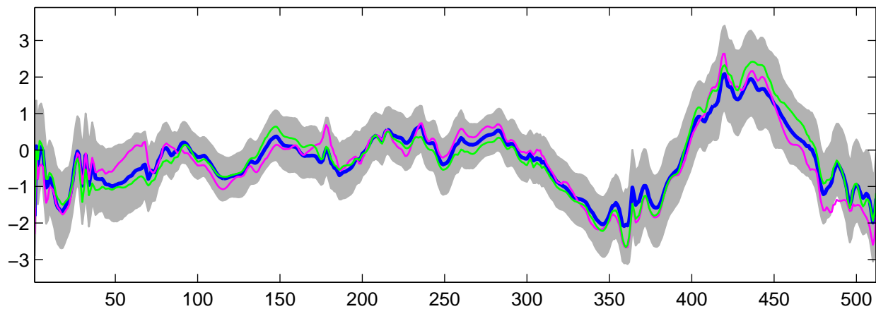
Estimated U_{24}(t) using G-WFMM: Normal data, run 1
