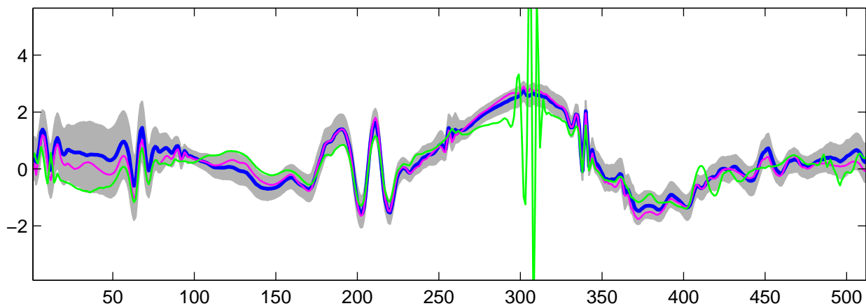
Estimated U_{24}(t) using R-WFMM: t_1 data, run 1
