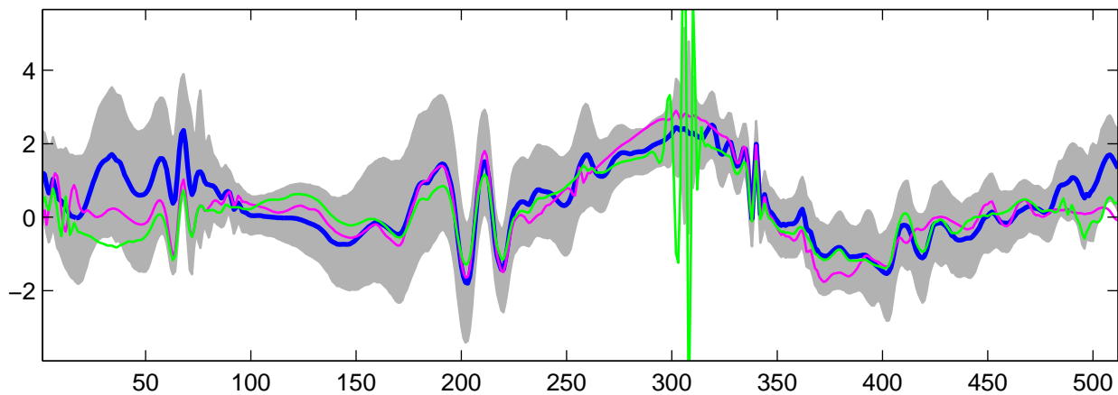
Estimated U_{24}(t) using G-WFMM: t_1 data, run 1
