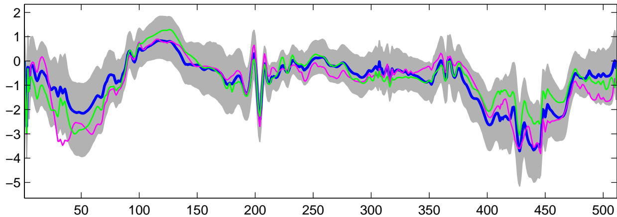
Estimated U_{24}(t) using G-WFMM: t_2 data, run 1
