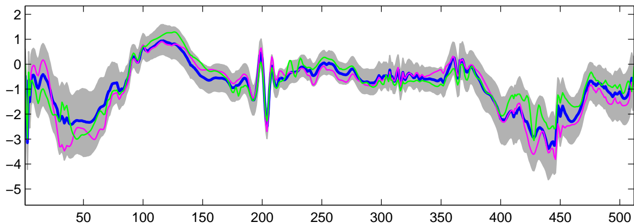
Estimated U_{24}(t) using R-WFMM: t_2 data, run 1
