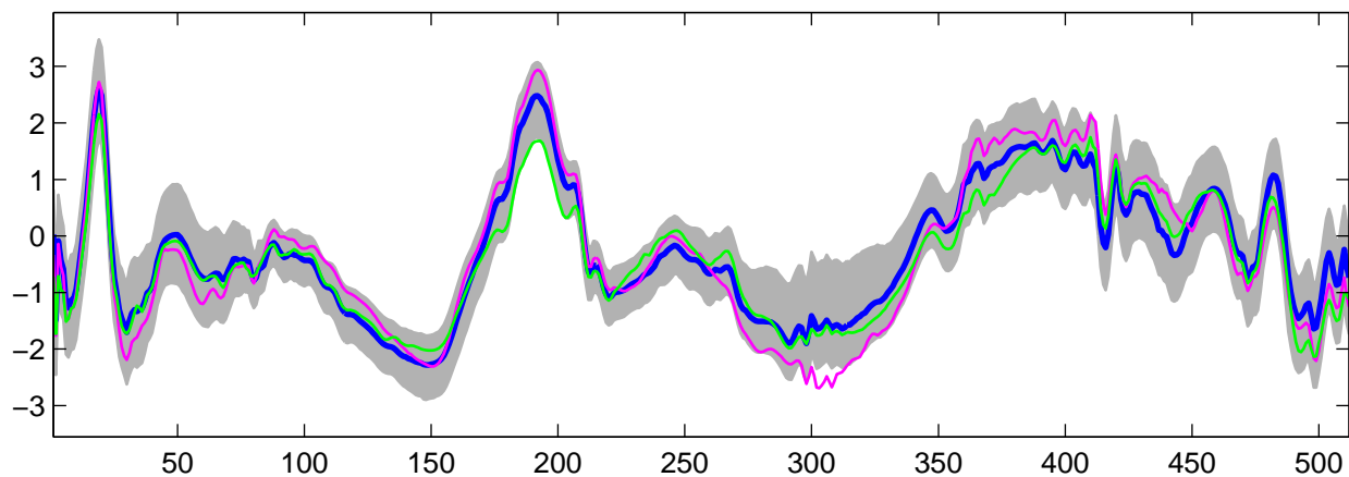
Estimated U_{24}(t) using R-WFMM: t_3 data, run 1
