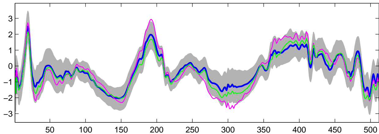
Estimated U_{24}(t) using G-WFMM: t_3 data, run 1
