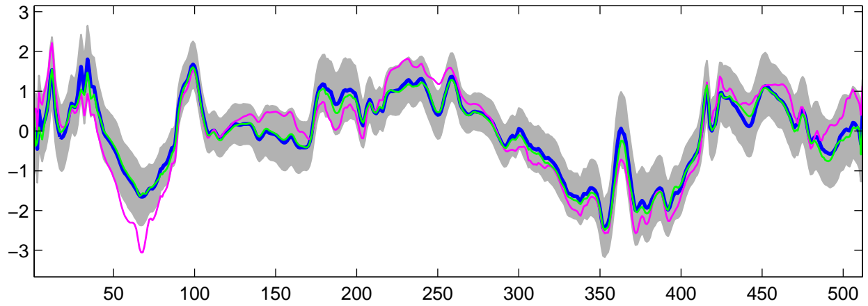
Estimated U_{25}(t) using G-WFMM: DE data, run 1
