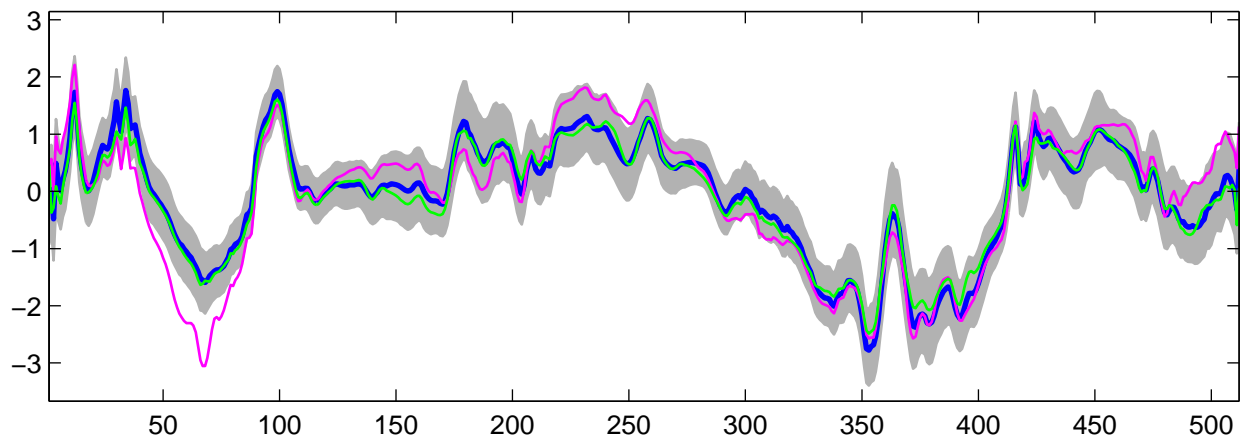
Estimated U_{25}(t) using R-WFMM: DE data, run 1
