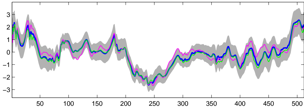
Estimated U_{25}(t) using G-WFMM: Normal data, run 1
