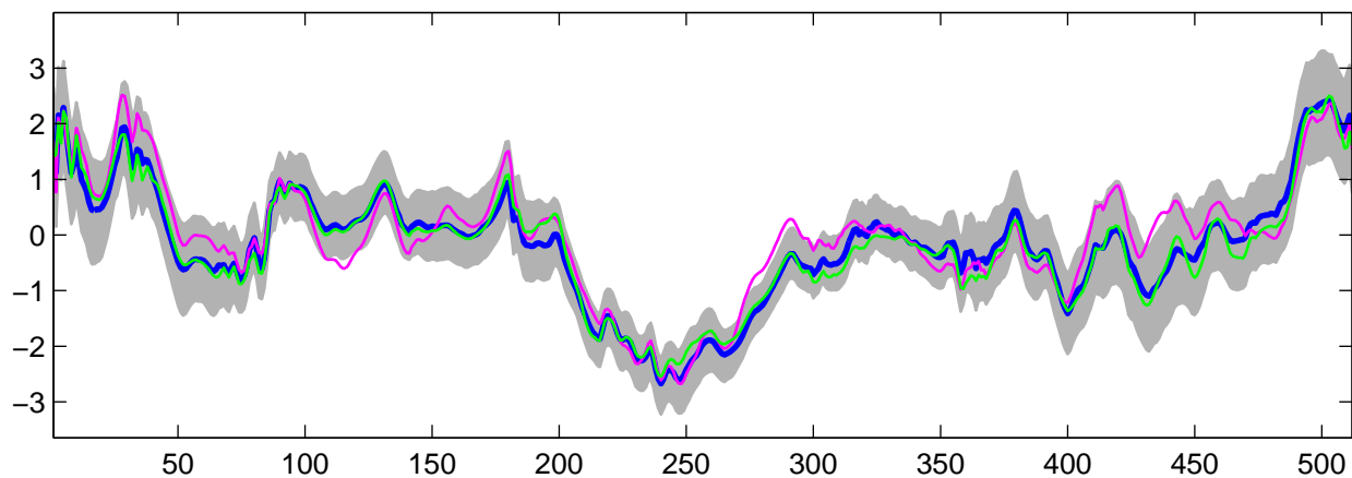
Estimated U_{25}(t) using R-WFMM: Normal data, run 1
