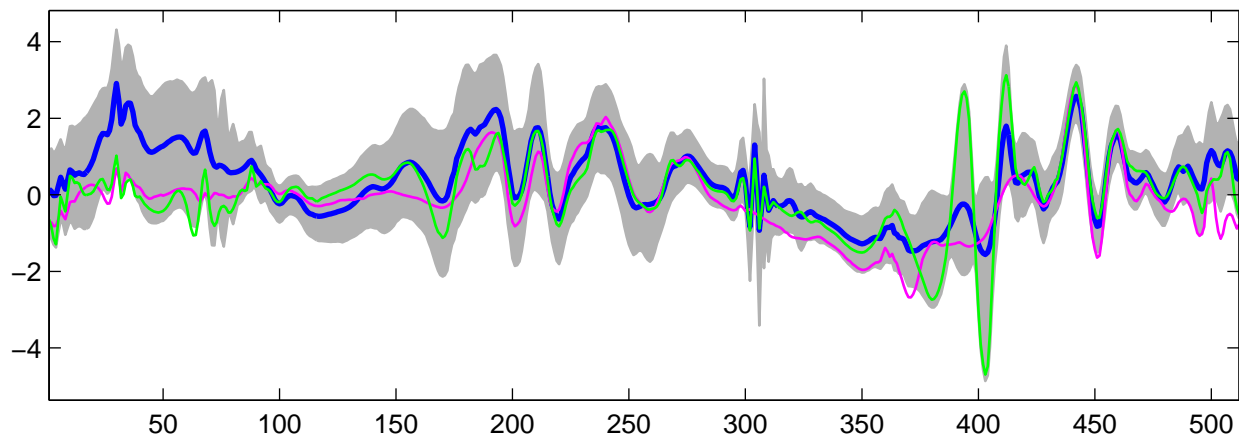
Estimated U_{25}(t) using G-WFMM: t_1 data, run 1
