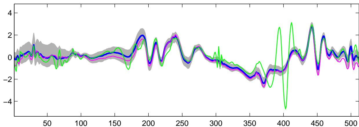
Estimated U_{25}(t) using R-WFMM: t_1 data, run 1
