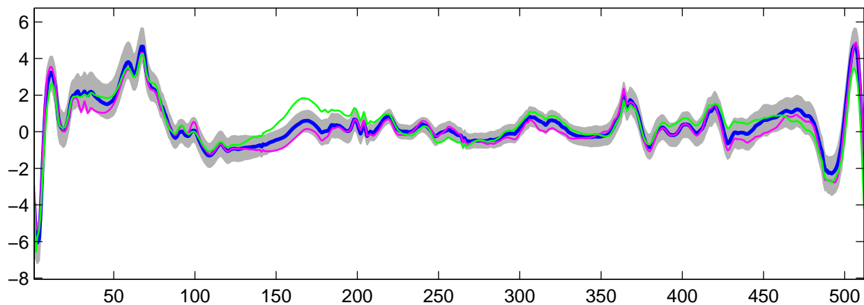
Estimated U_{25}(t) using R-WFMM: t_2 data, run 1
