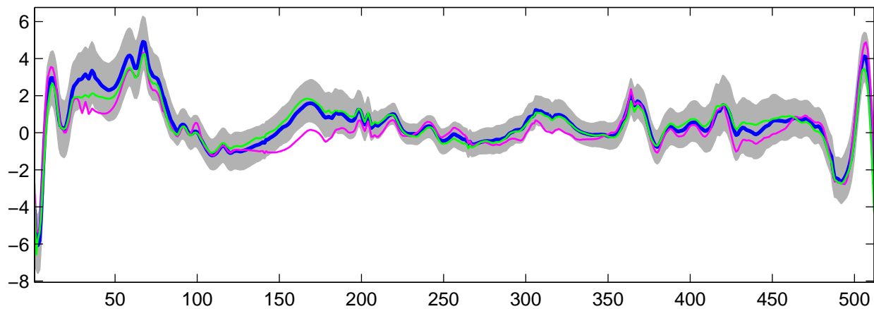
Estimated U_{25}(t) using G-WFMM: t_2 data, run 1
