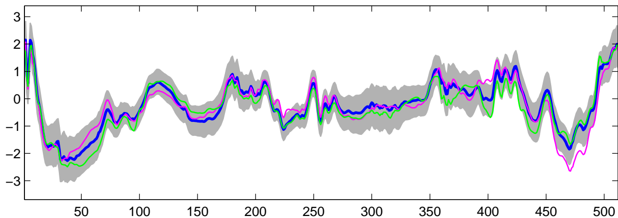
Estimated U_{25}(t) using R-WFMM: t_3 data, run 1
