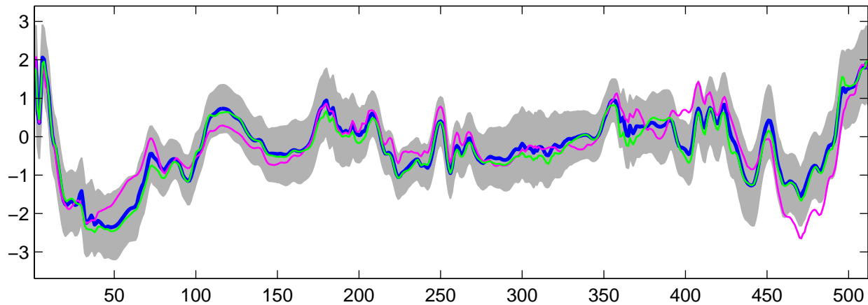
Estimated U_{25}(t) using G-WFMM: t_3 data, run 1
