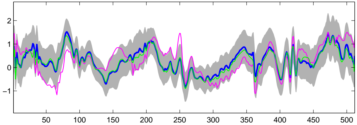
Estimated U_{26}(t) using G-WFMM: DE data, run 1
