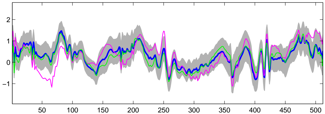
Estimated U_{26}(t) using R-WFMM: DE data, run 1
