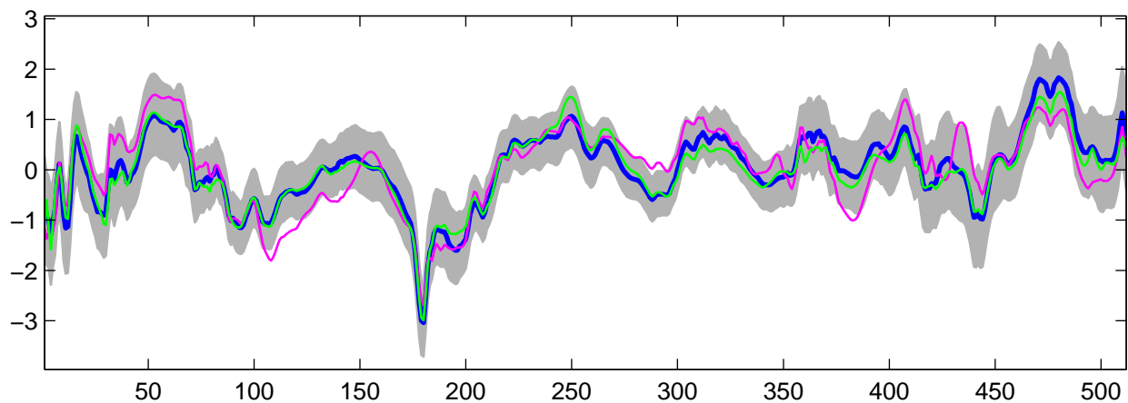
Estimated U_{26}(t) using R-WFMM: Normal data, run 1
