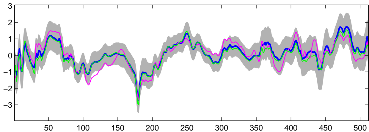
Estimated U_{26}(t) using G-WFMM: Normal data, run 1
