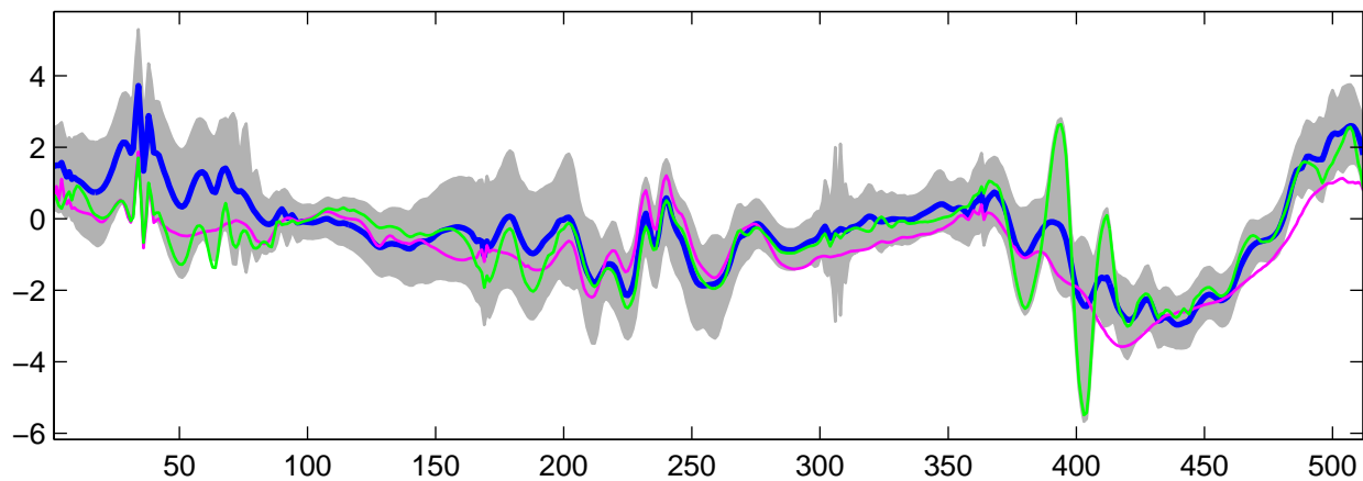
Estimated U_{26}(t) using G-WFMM: t_1 data, run 1
