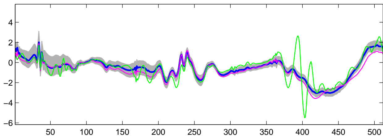
Estimated U_{26}(t) using R-WFMM: t_1 data, run 1
